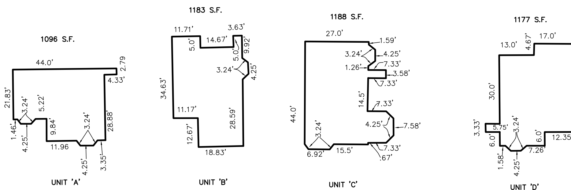
TYPICAL UNIT DIMENSIONS
