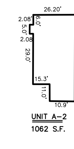
TYPICAL UNIT DIMENSIONS N.T.S.
