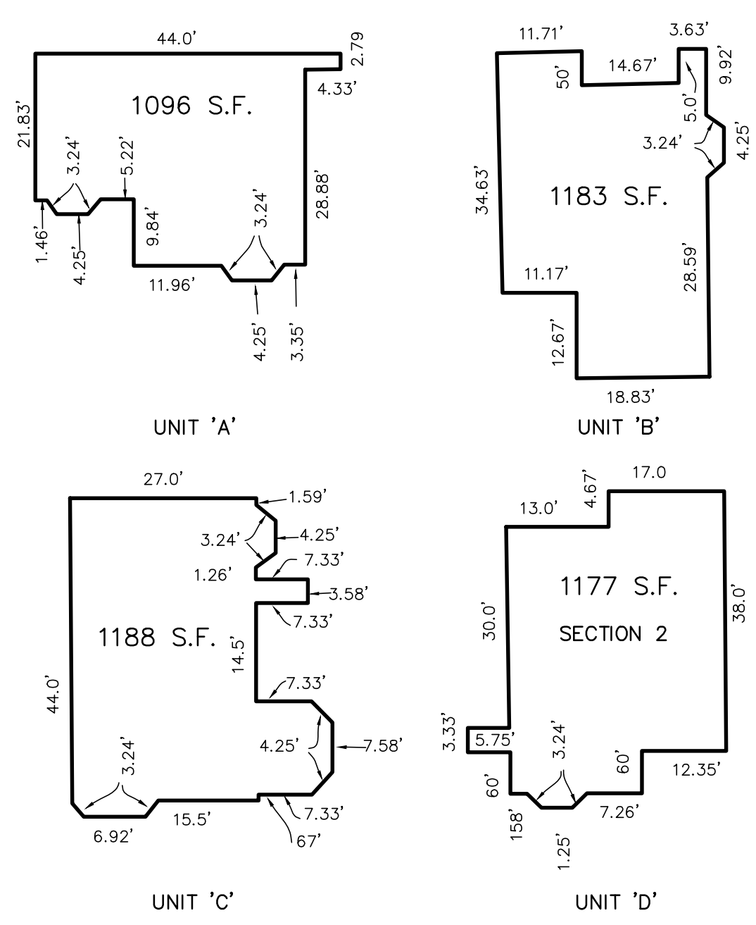
TYPICAL UNIT DIMENSIONS
